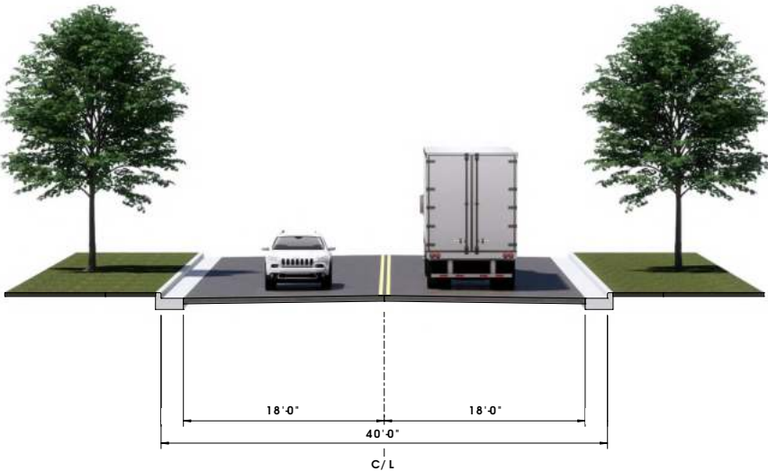
existing typical section County B (Fantasia Reed Road) to Airport Road
