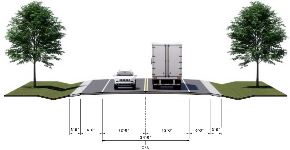
existing typical section County B (Bainbridge Street / Dawson Avenue) to County B (Fantasia Reed Road)
