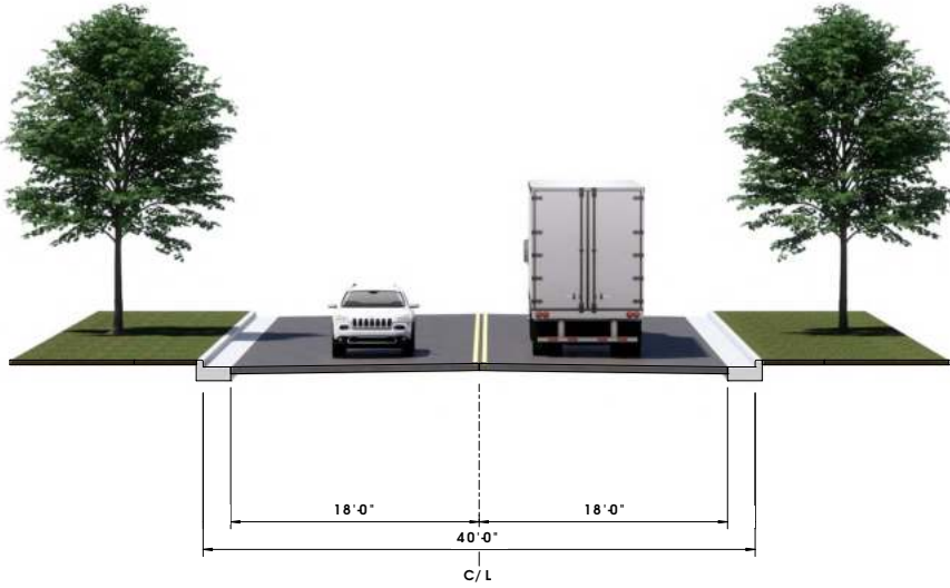
existing typical section County B (Clinton Street) to County B (Bainbridge Street)
