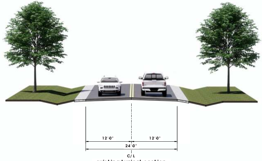
existing typical section Airport Road to County B W (Lakeshore Drive)
